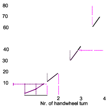
Flow regulation diagram Qn = 80 l/min ; P = 100 bar
