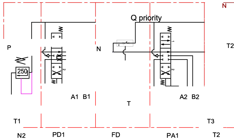
Hydraulic circuit
